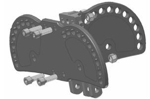
Fig 20 Half Plate attachment to Main Plate
