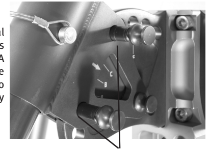
Fig 4 Load Locking Head Pins (Parked position)
